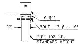
PLAN OF BRACKET "A"
