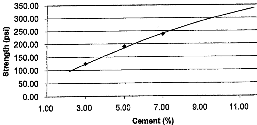
% Cement vs Strength (psi)
