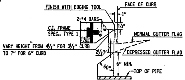
DETAIL AT WEIR
