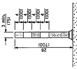
FLEXIBLE DELINEATOR
