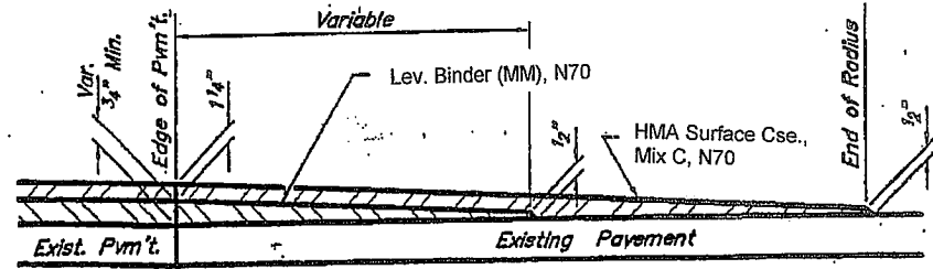
SECTION A-A SIDE ROAD
