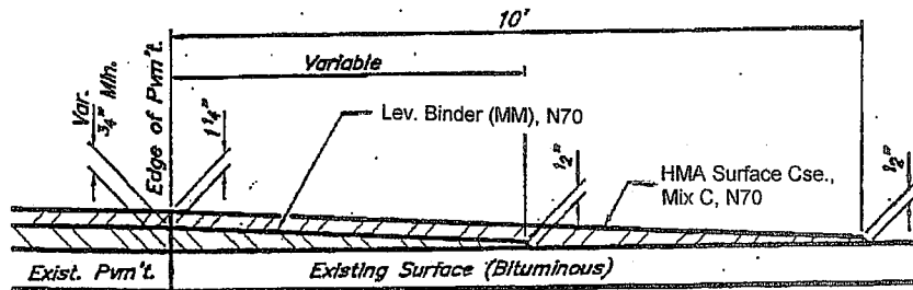
SECTION A-A PRIVATE ENTRANCE
