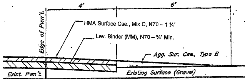
SECTION A-A PRIVATE ENTRANCE - GRAVEL
