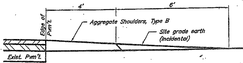
SECTION A-A FIELD ENTRANCE
