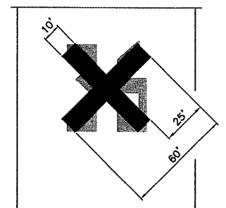
ON PAVEMENT CLOSED RUNWAY MARKER DETAIL NO SCALE
