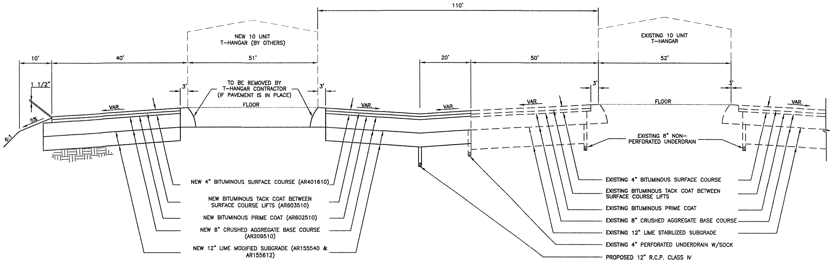
T-HANGAR AND TAXILANE SECTION A-A N.T.S.
