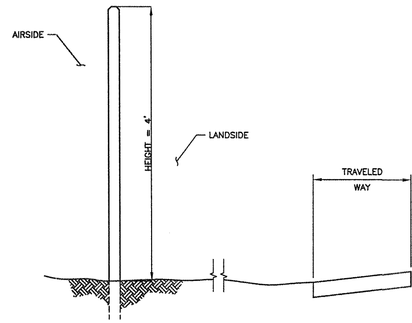
BARBED WIRE EXTENSION BRACKET N.T.S.
