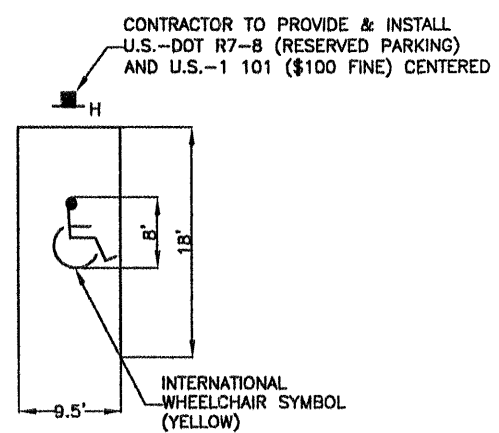
HANDICAP PARKING SPACE N.T.S.
