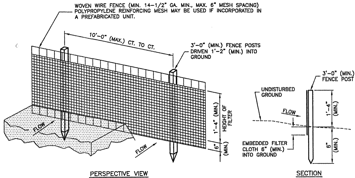
EROSION CONTROL FABRIC FENCE DETAIL N.T.S.
