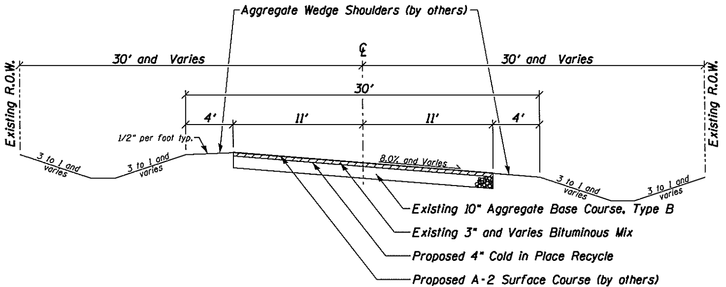
Typical Cross Section (Superelevation) Station 261+34.5 to 268+39.50
