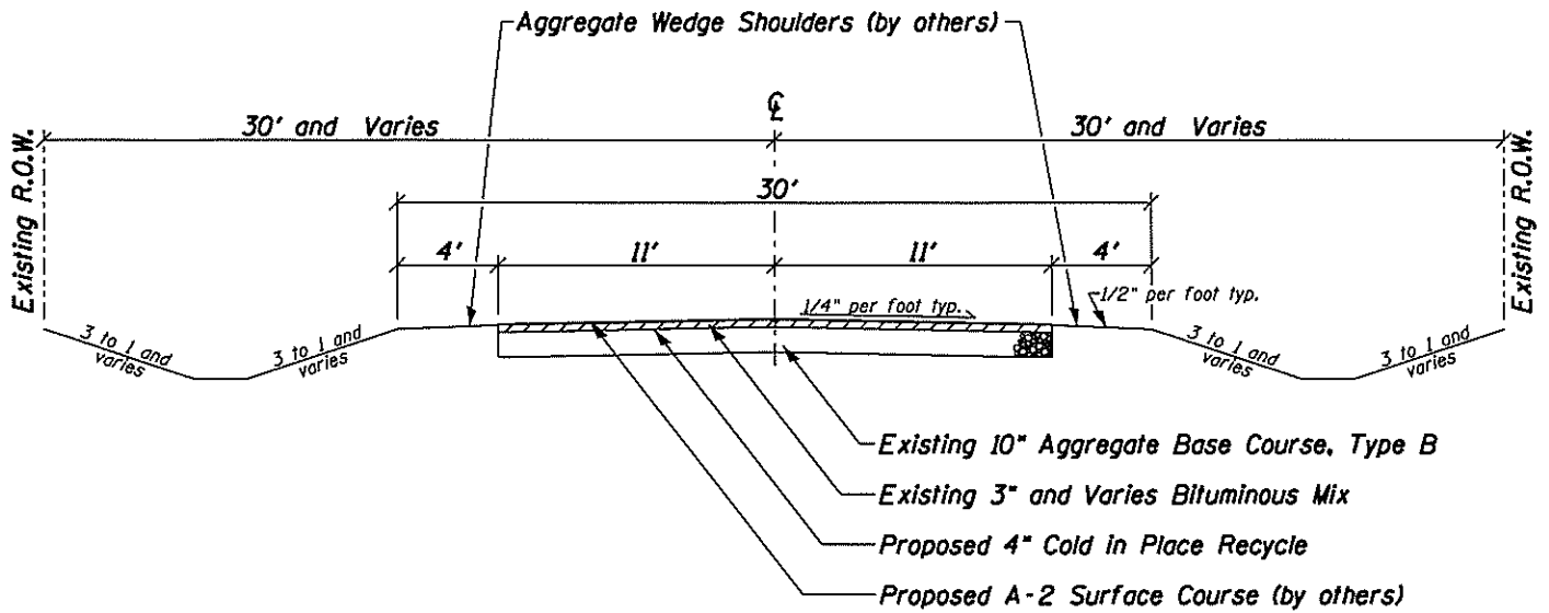
Typical Cross Section (Normal Crown) Station 0+00 to 261+34.5
