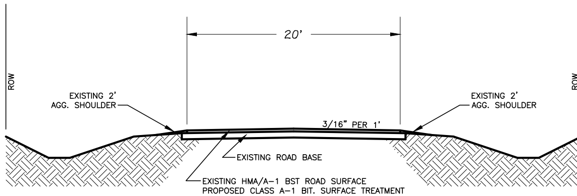
TYPICAL CROSS SECTION OF EXISTING/PROPOSED ROAD
