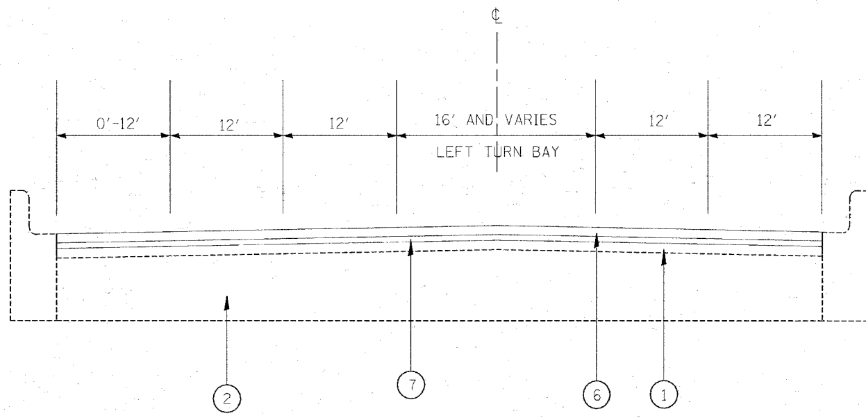
LAKE STREET PROPOSED TYPICAL SECTION STA. 50+00 TO STA. 60+00
