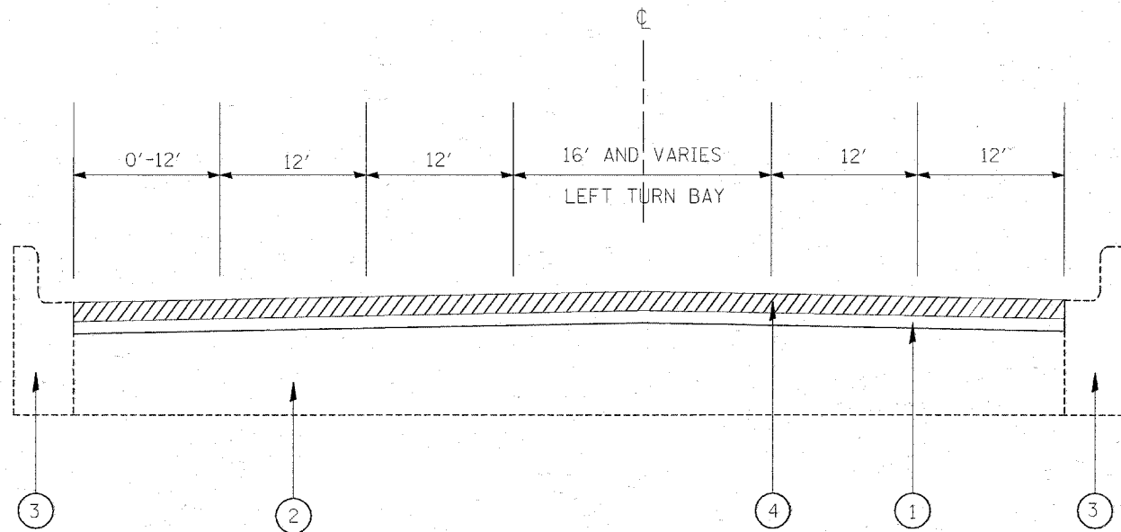
LAKE STREET EXISTING TYPICAL SECTION STA. 50+00 TO STA. 60+00
