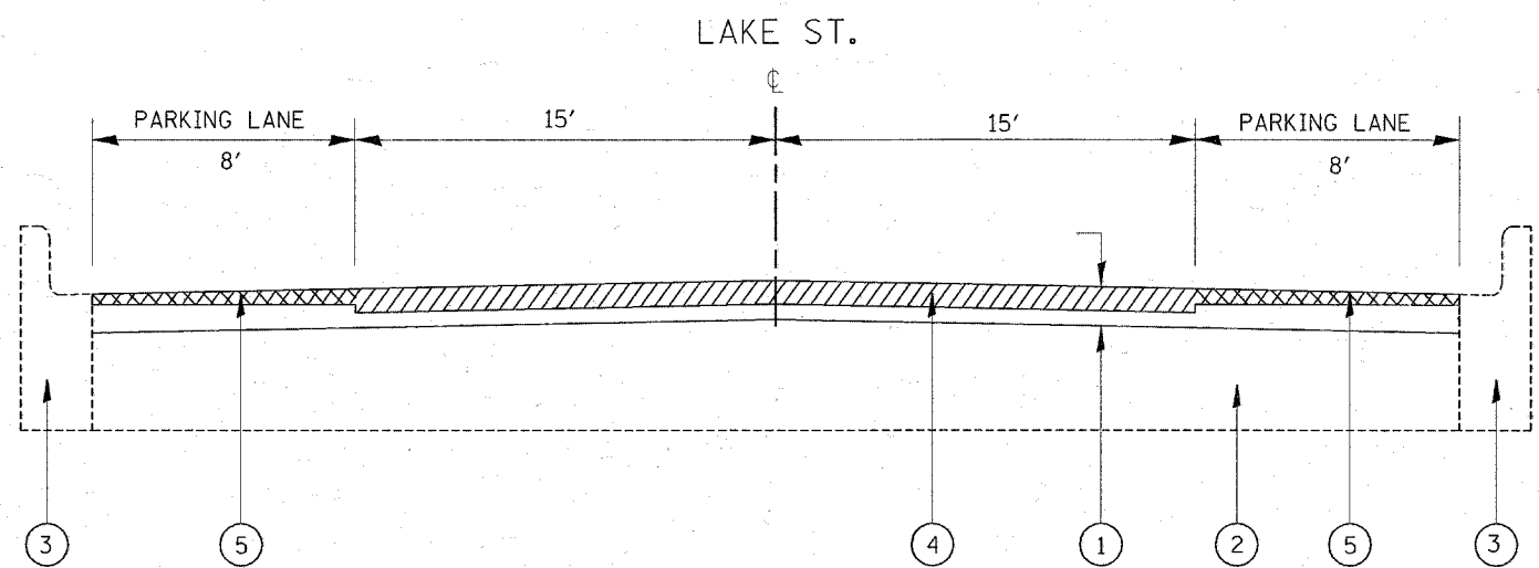
LAKE STREET EXISTING TYPICAL SECTION STA. 60+00 TO STA. 135+95
