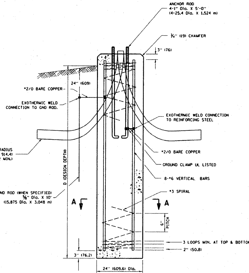
FOUNDATION DETAIL
