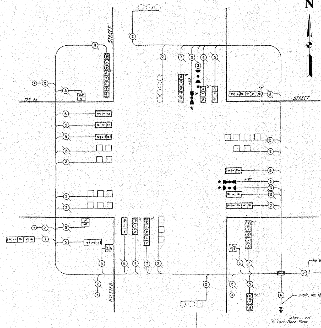
CABLE PLAN
