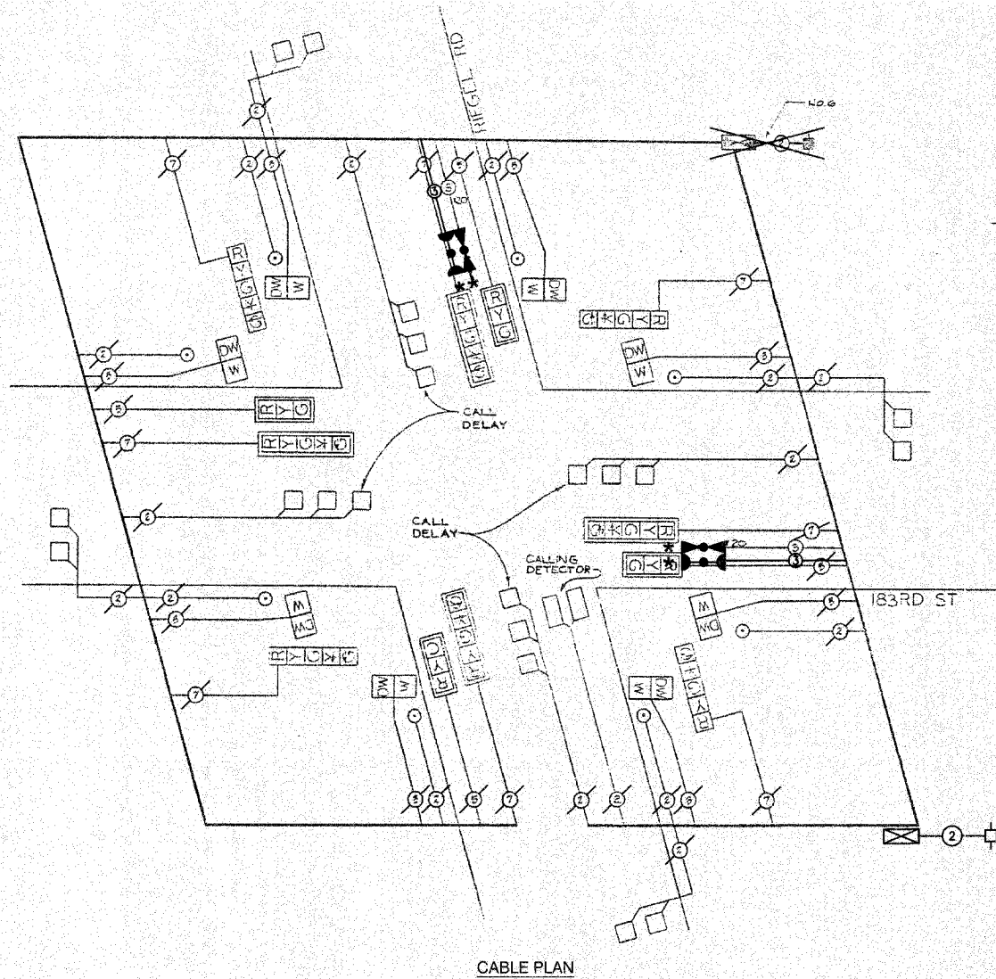
CABLE PLAN
