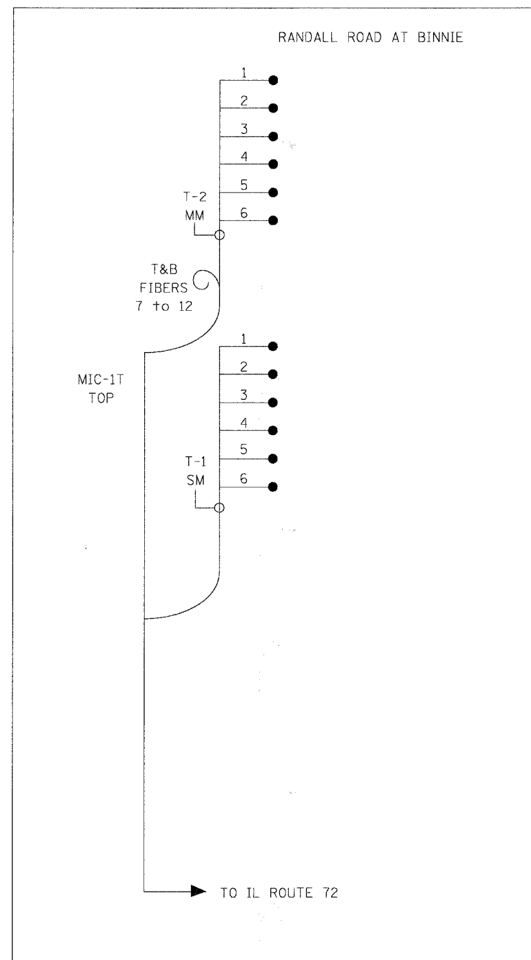
TERMINATION PLAN 6
