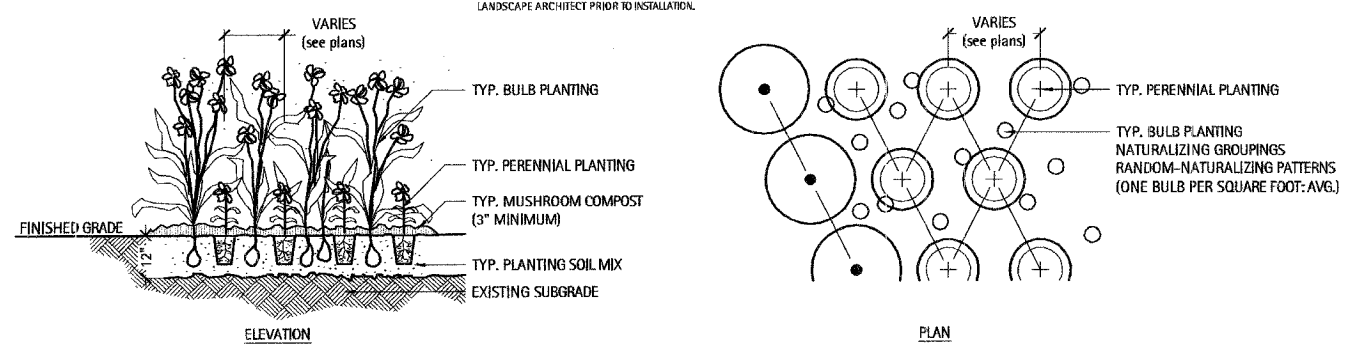
2 Typical Groundcover & Perennial Planting Detail Scale: NTS
