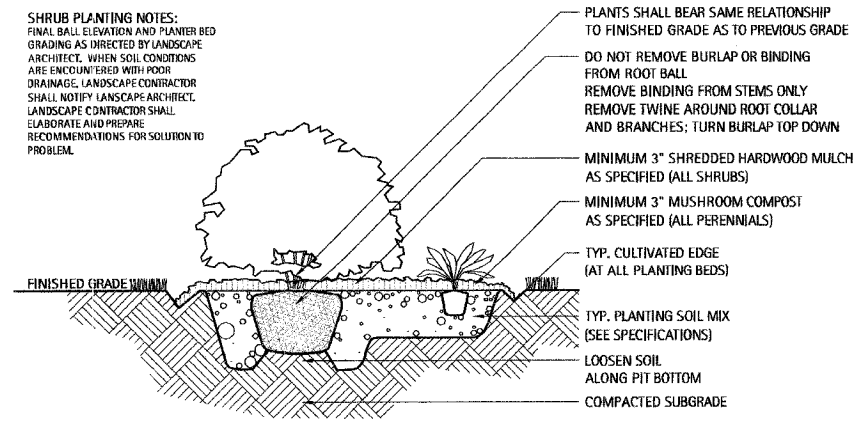
1 Typical Shrub Planting Detail Scale: NTS
