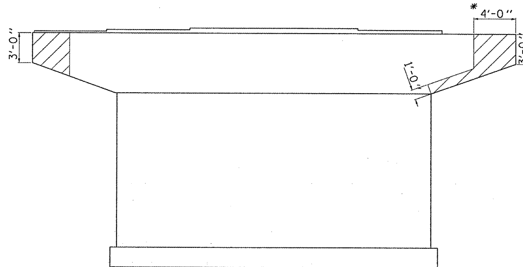
PIER #3 NORTH FACE
