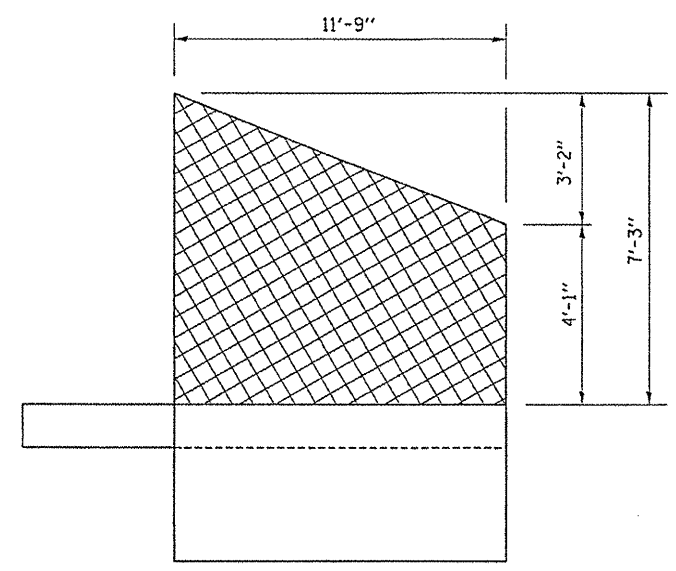
ELEVATION (TYPICAL)
