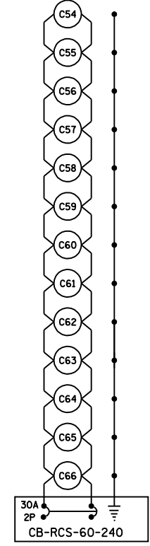
CONTROLLER 4 CKT A ALL *2 UNIT DUCT
