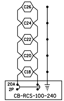
CONTROLLER 1 CKT D ALL *6 UNIT DUCT
