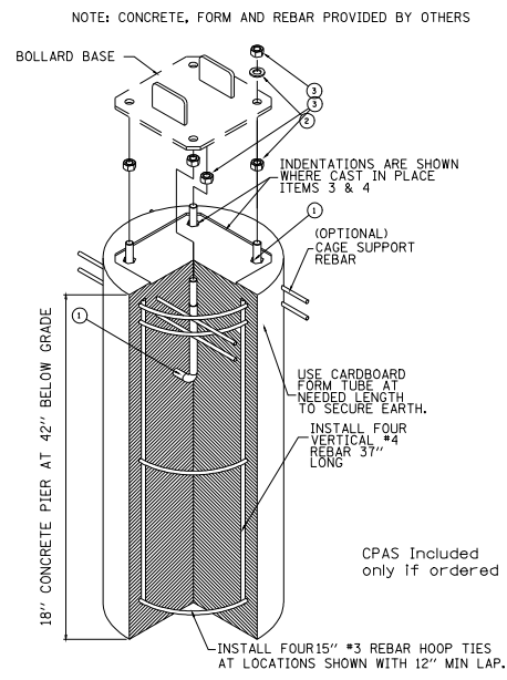
CONCRETE PIER ANCHOR SYSTEM FOR DROP GATE
