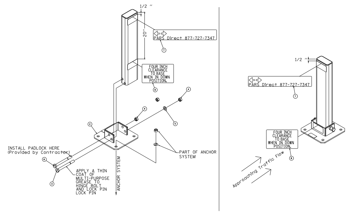
DROP GATE INSTALLATION DETAIL
