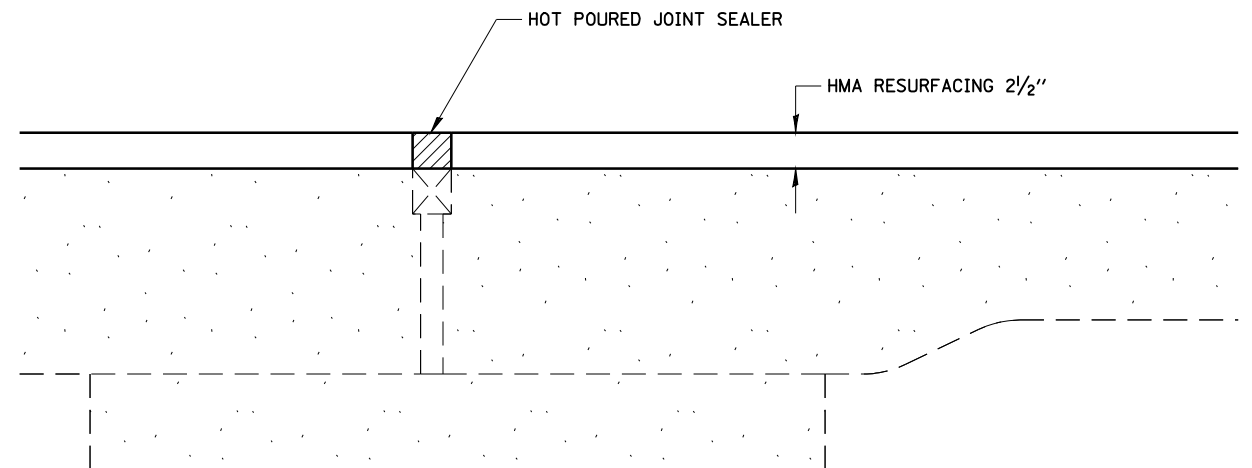
PREFORMED JOINT SEAL TREATMENT SECTION A-A (AT PREFORMED JOINT)
