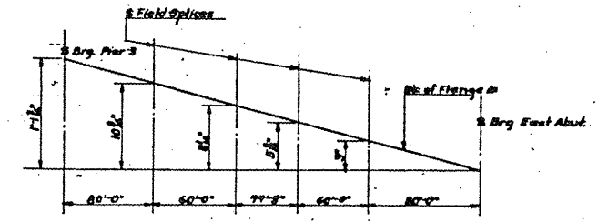
FABRICATION DIAGRAM
