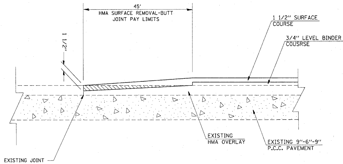
BRIDGE OMISSION DETAIL
