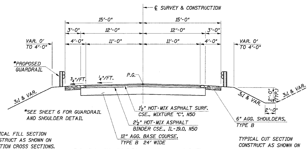
PROPOSED TYPICAL CROSS SECTION
