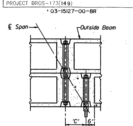
PARTIAL PLAN TRANSVERSE TIE ASSEMBLY (D=15°, 20°, 25° and 30°)
