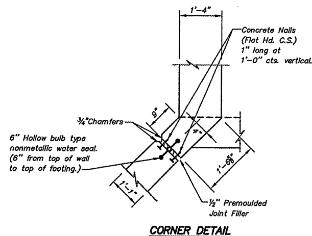
CORNER DETAIL
