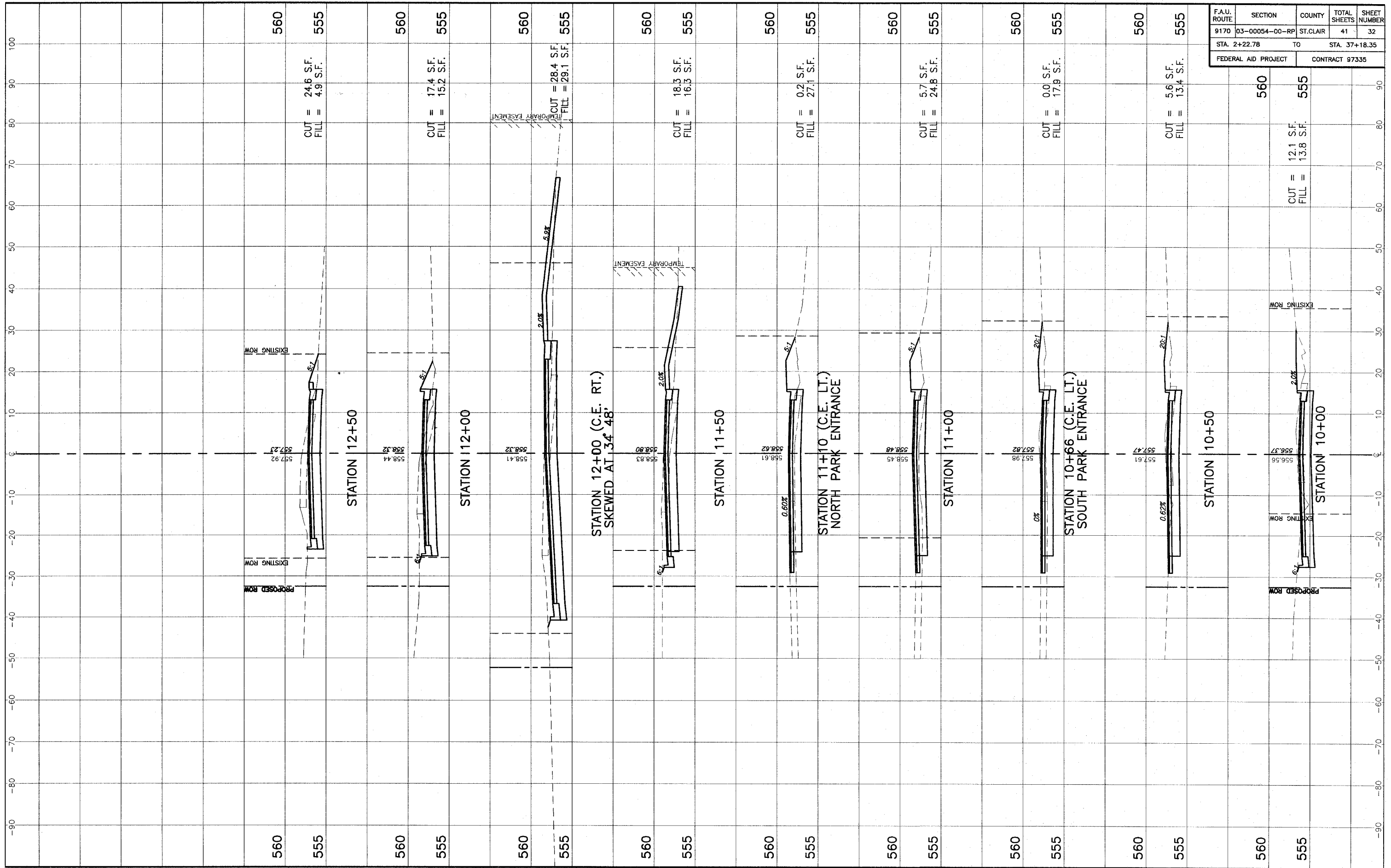
STA. 10+00 - STA. 12+50 CROSS SECTIONS OBERNEUEFEMANN ROAD IMPROVEMENTS SECTION 03-00054-00-RP ST. CLAIR COUNTY, ILLINOIS
