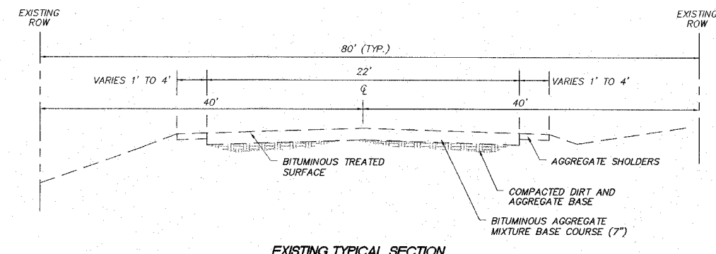
EXISTING TYPICAL SECTION STAMPER LANE
