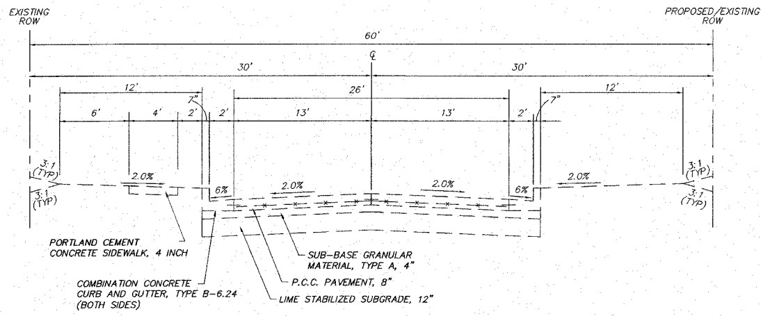
EXISTING TYPICAL SECTION STA 67+49.80
