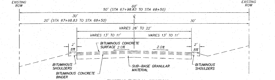
EXISTING TYPICAL SECTION STA 67+49.80 TO STA 68+50
