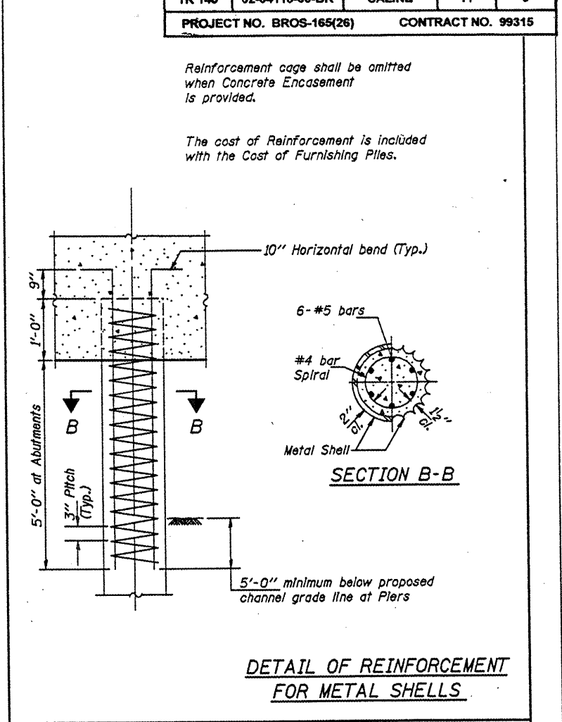
DETAIL OF REINFORCEMENT FOR METAL SHELLS
