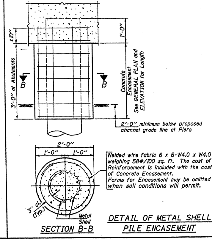
DETAIL OF REINFORCEMENT FOR METAL SHELLS
