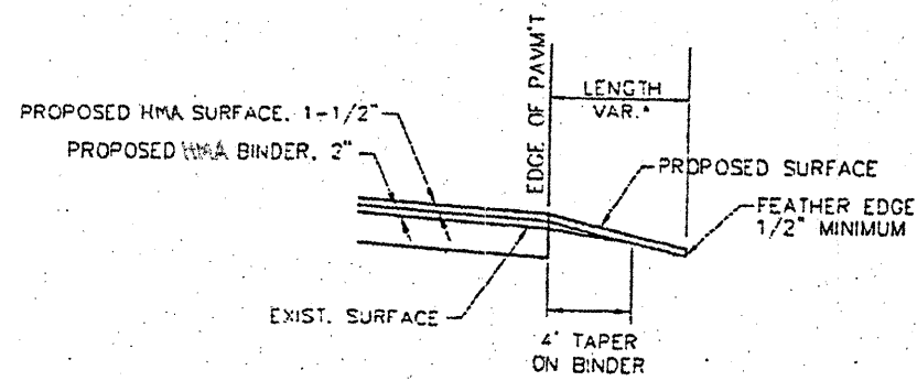
SIDEROAD DETAILS
