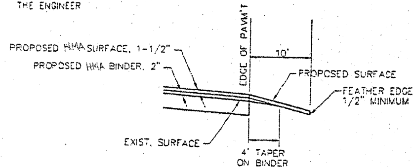
PRIVATE ENTRANCE DETAILS
