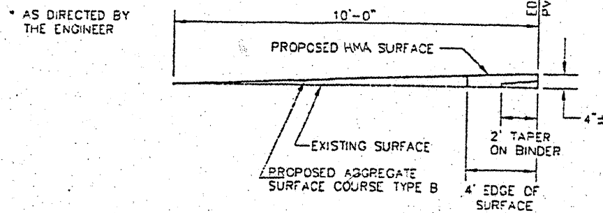
FIELD ENTRANCE DETAILS
