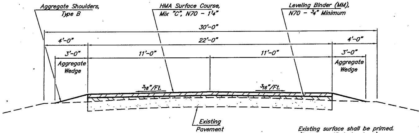
TYPICAL SECTION
