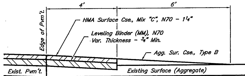
SECTION A-A PRIVATE ENTRANCE - AGGREGATE (Est. No. = 50)
