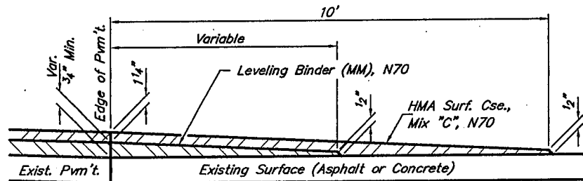
SECTION A-A PRIVATE ENTRANCE - ASPHALT (Est. No. = 5)
