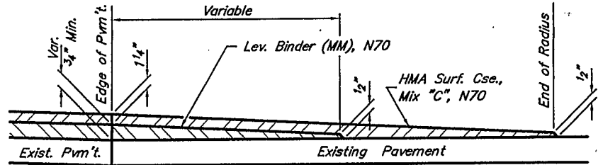
SECTION A-A SIDE ROAD (Est. No. = 10)
