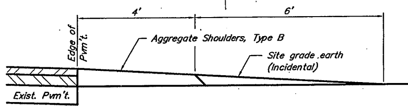
SECTION A-A FIELD ENTRANCE (Est. No. = 44)
