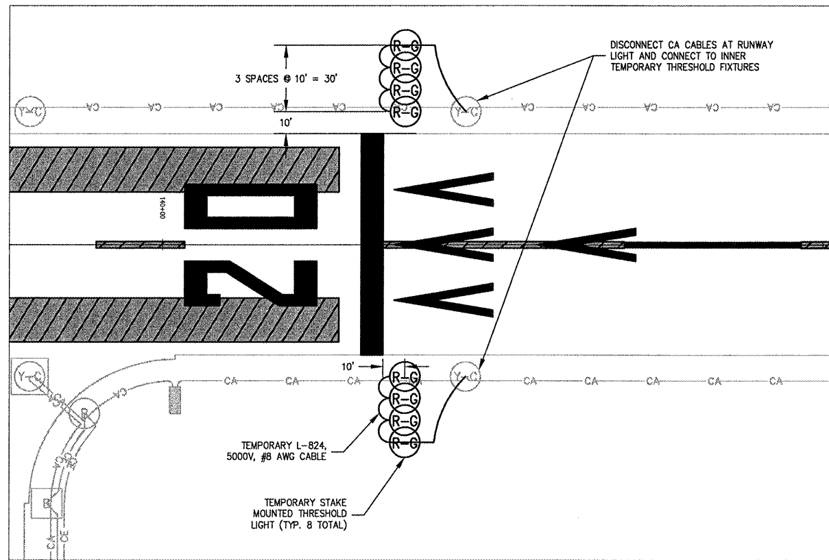
TEMPORARY RUNWAY 20 THRESHOLD - LIGHTING
