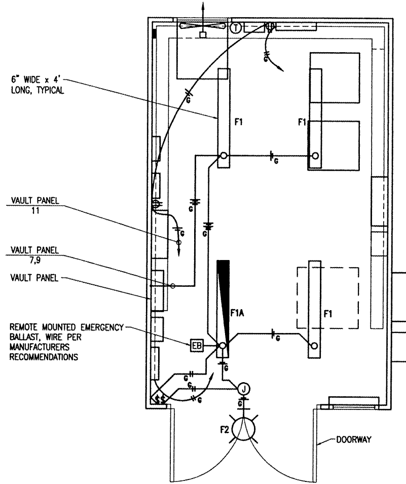
VAULT LIGHTING & RECEPTACLE PLAN SCALE 1/2"=1'-0" 1 0 2 4 FEET
