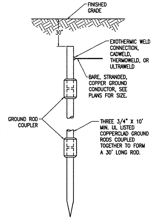
30 FT. GROUND ROD
