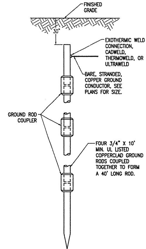
40 FT. GROUND ROD
