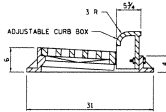
TRANSVERSE SECTION
