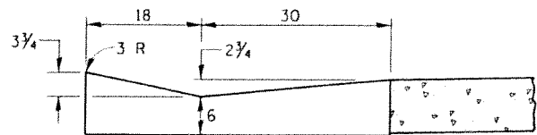
Section B-B
