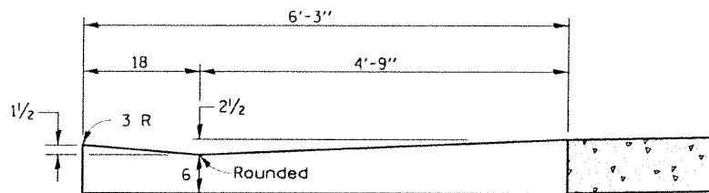
Section C-C
