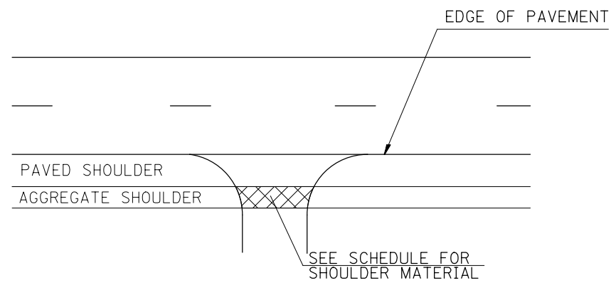
SIDEROAD DETAIL
