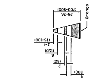
REFLECTORIZED CONE
