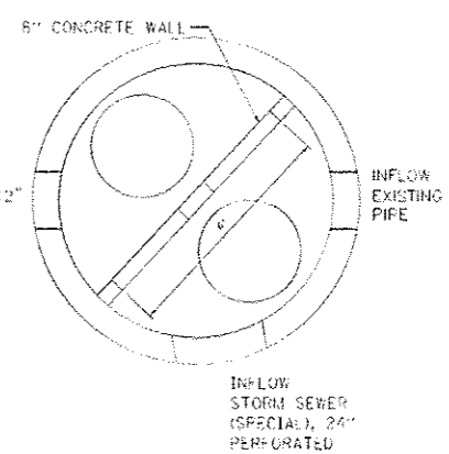
MANHOLE TYPE A, 6' DIA. TYPE I FRAME AND OPEN LID. SPECIAL DETAIL NOT TO SCALE
