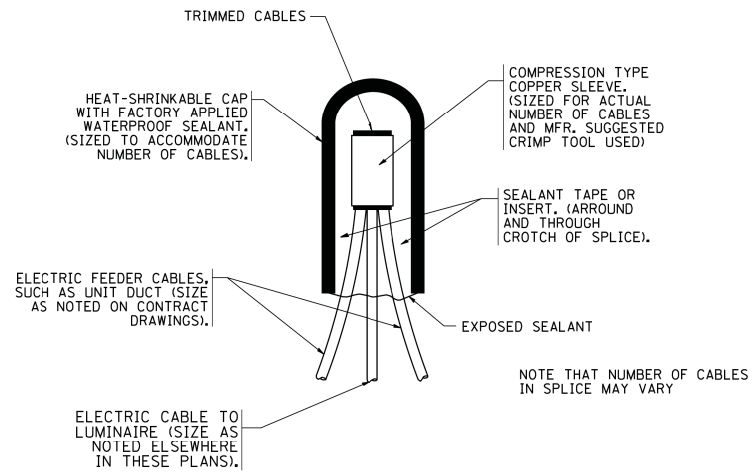
TYPICAL SPLICE DETAIL N.T.S.
