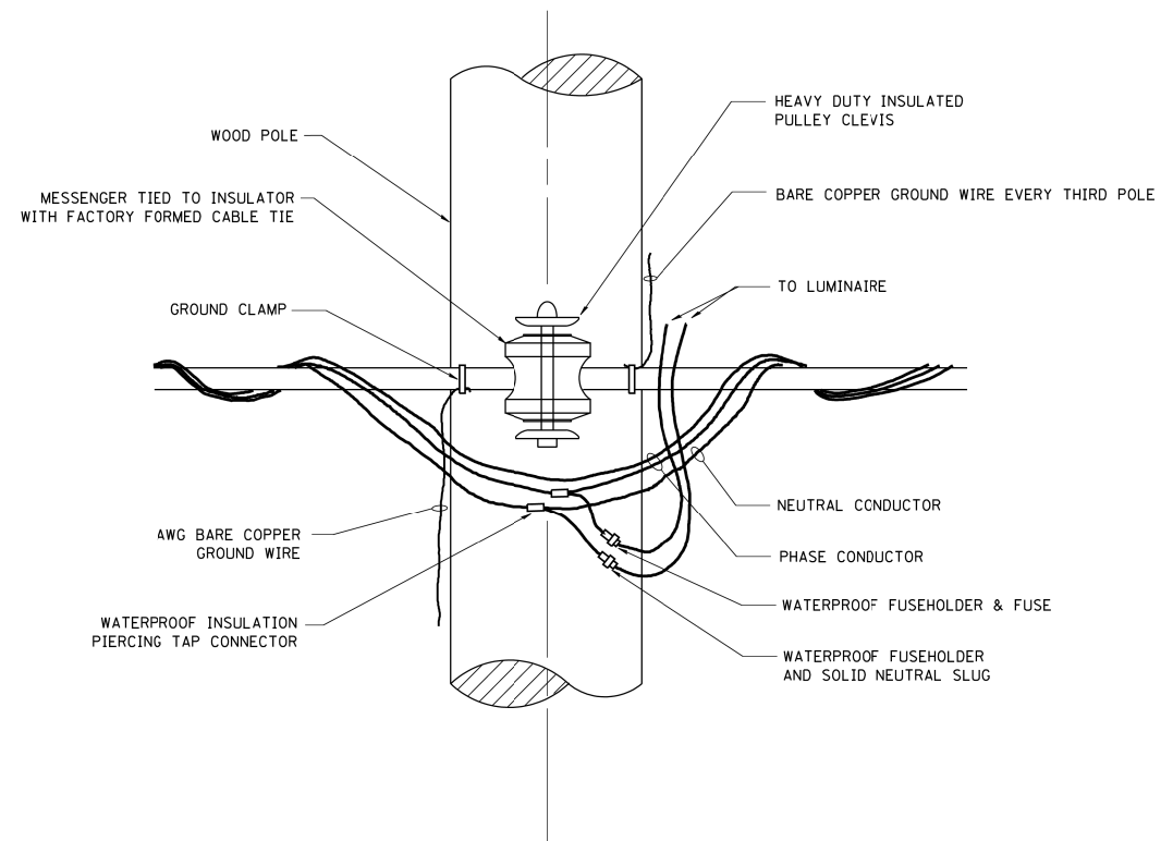
TEMPORARY LIGHT POLE ATTACHMENT DETAIL
