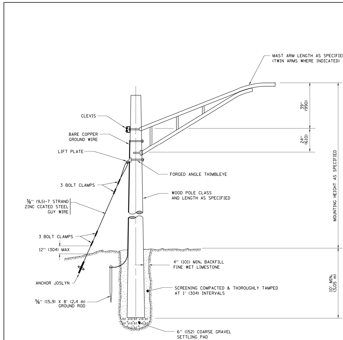
TEMPORARY LIGHT POLE DETAIL
