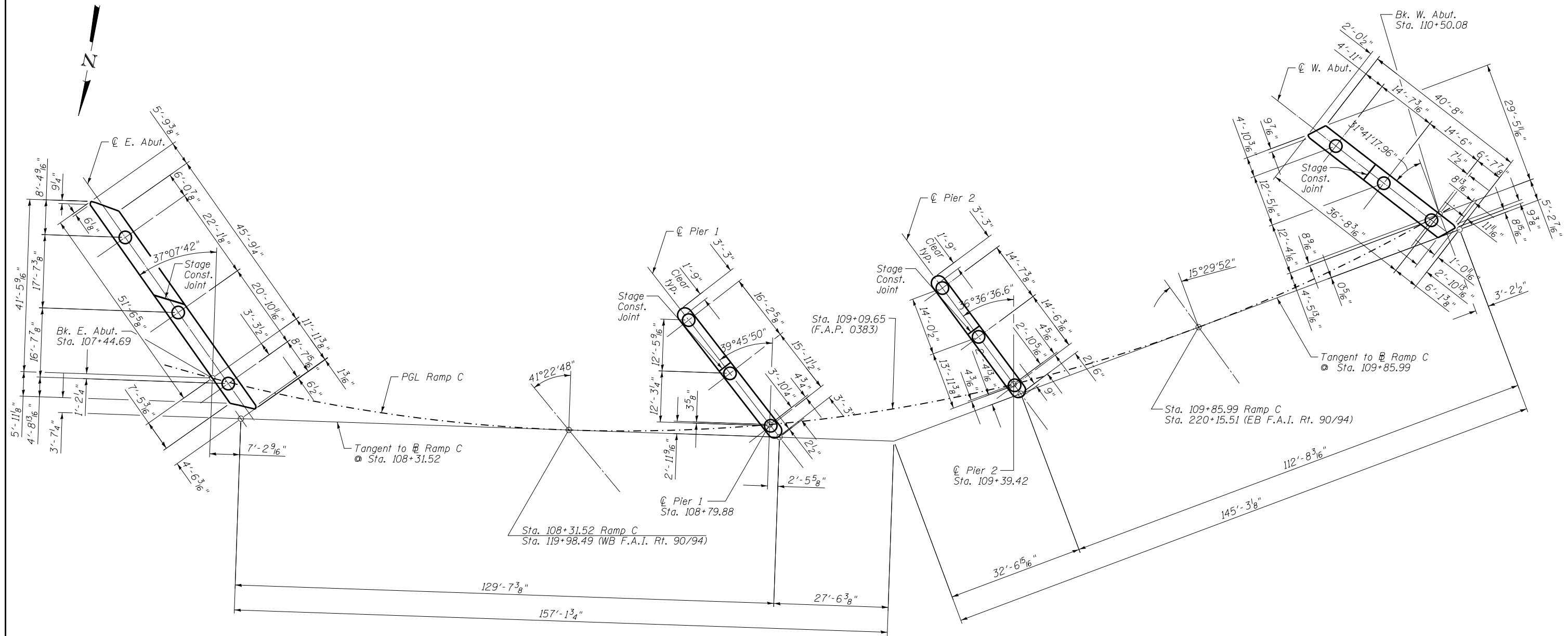
SUBSTRUCTURE LAYOUT PLAN
