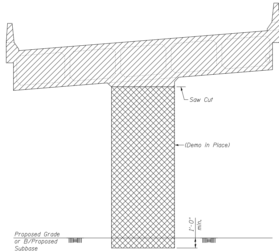
TYPICAL SECTION AT PIER WITH SPMT REMOVAL OF SUPERSTRUCTURE
