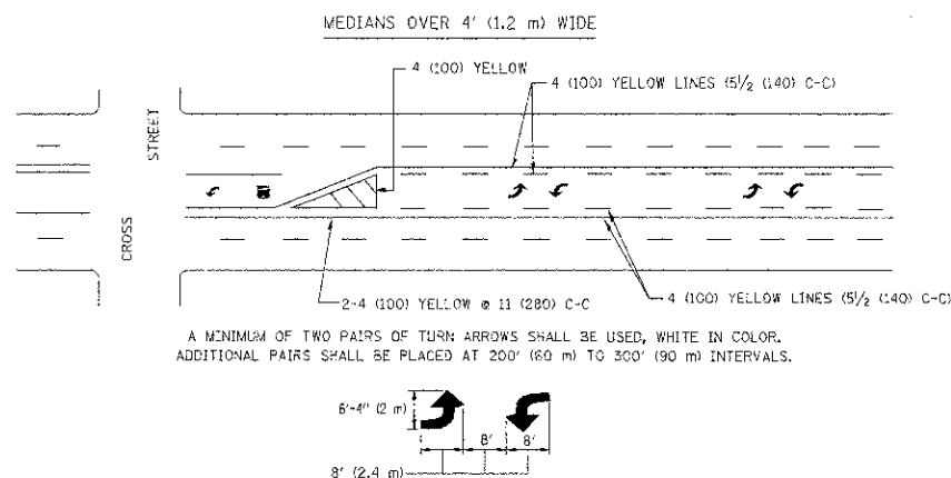
MEDIAN WITH TWO-WAY LEFT TURN LANE
