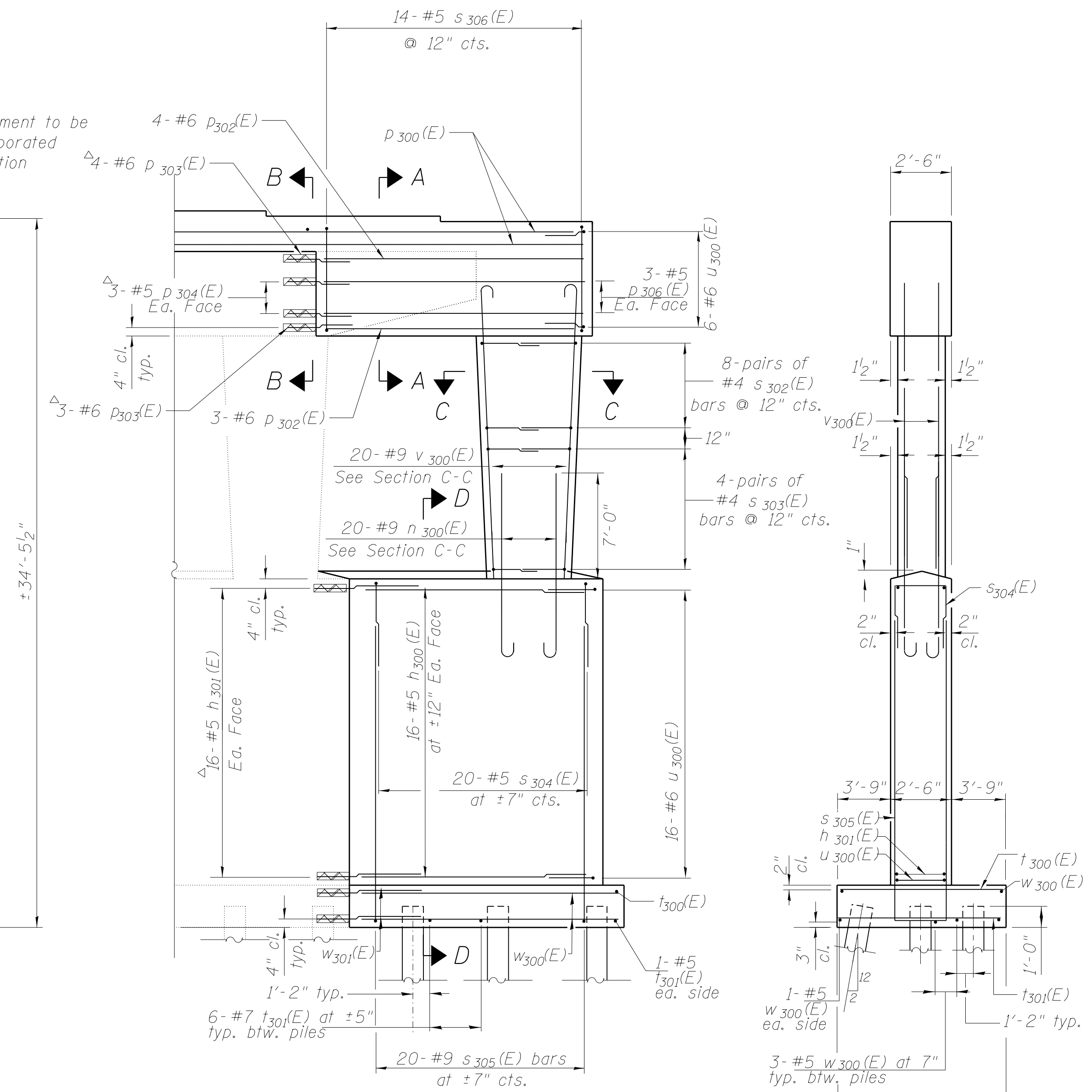
PARTIAL ELEVATION - NORTH END
