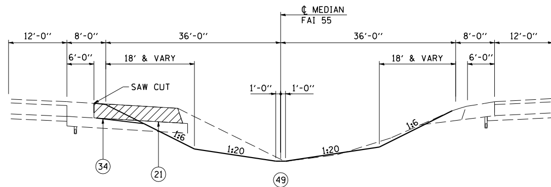
FAI ROUTE 55 FINAL PHASE TYPICAL CROSS SECTIONS SN 054-0065, 0066, 0067, 0068 (47) STA 484+52.78 TO STA 487+61.92
