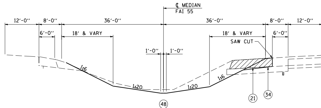
FAI ROUTE 55 FINAL PHASE TYPICAL CROSS SECTIONS SN 054-0065, 0066, 0067, 0068 (47) STA 479+77.84 TO STA 482+08.12 (47)
