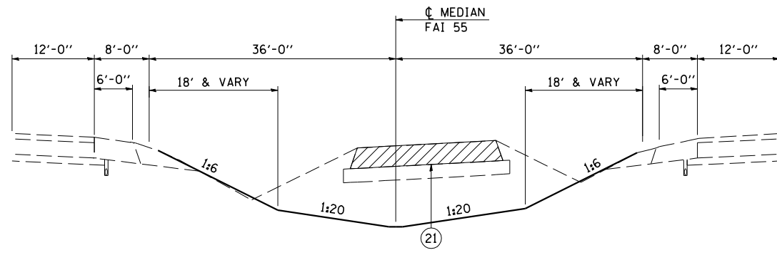
FAI ROUTE 55 FINAL PHASE TYPICAL CROSS SECTIONS SN 054-0065, 0066, 0067, 0068 (46) STA 476+47.88 TO STA 479+77.84 (48) (48) STA 482+08.12 TO STA 484+52.78 (49)
