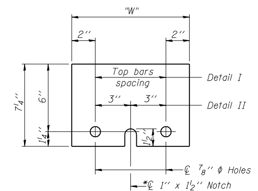
STEEL RETAINER PL 1" x 7 1/4" x "W"
