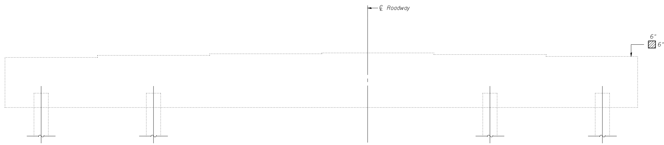
S.N. 054-0064 (S.B.) NORTH ABUTMENT ELEVATION (Looking North)
