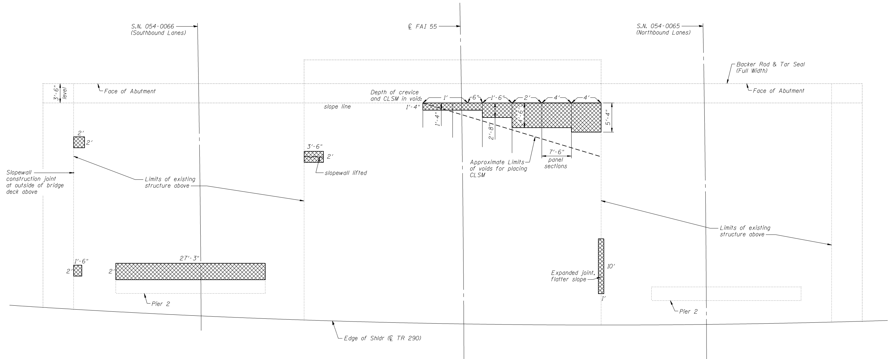
PLAN (Looking North)
