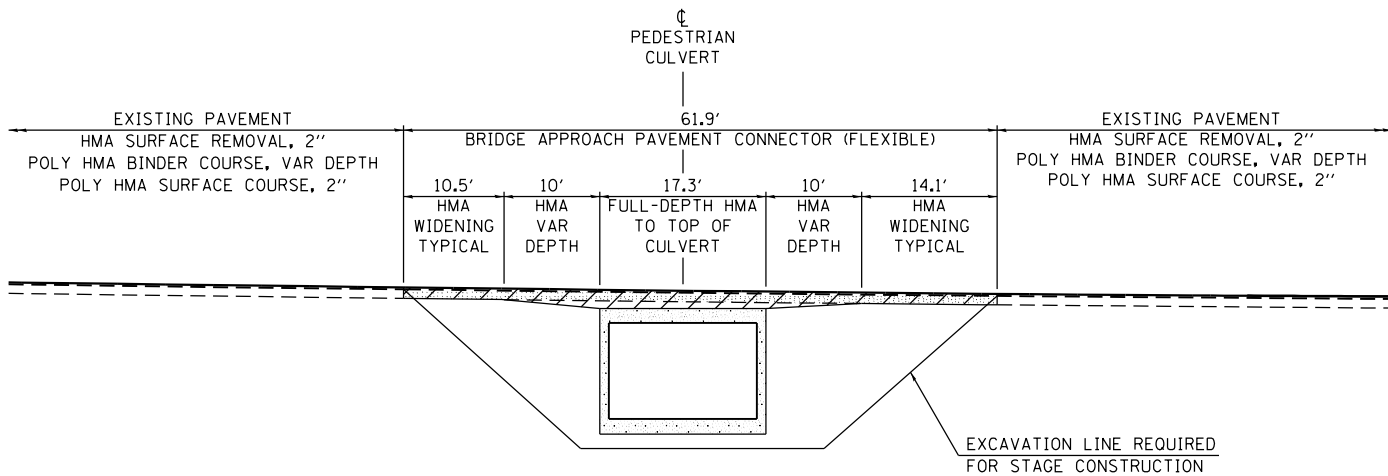
BRIDGE APPROACH PAVEMENT CONNECTOR (FLEXIBLE)
