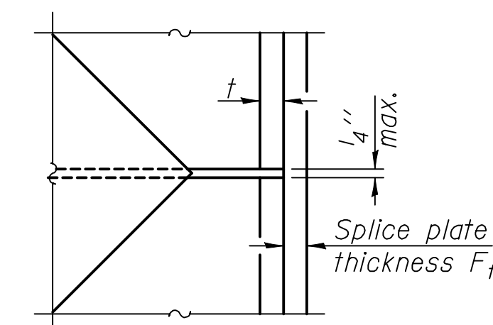
DETAIL D
